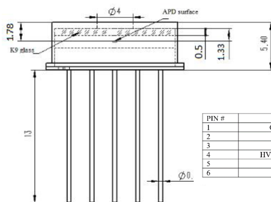
Pin description
