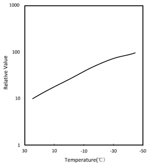
Time Constant vs. Temperature
