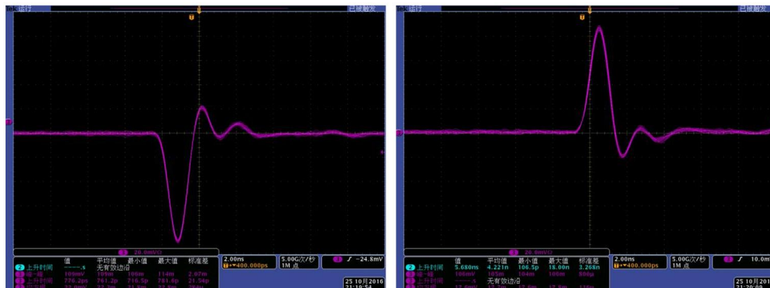
Frequency Response (inverting input)
