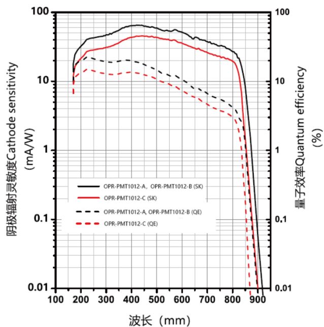
Typical spectral response curve
